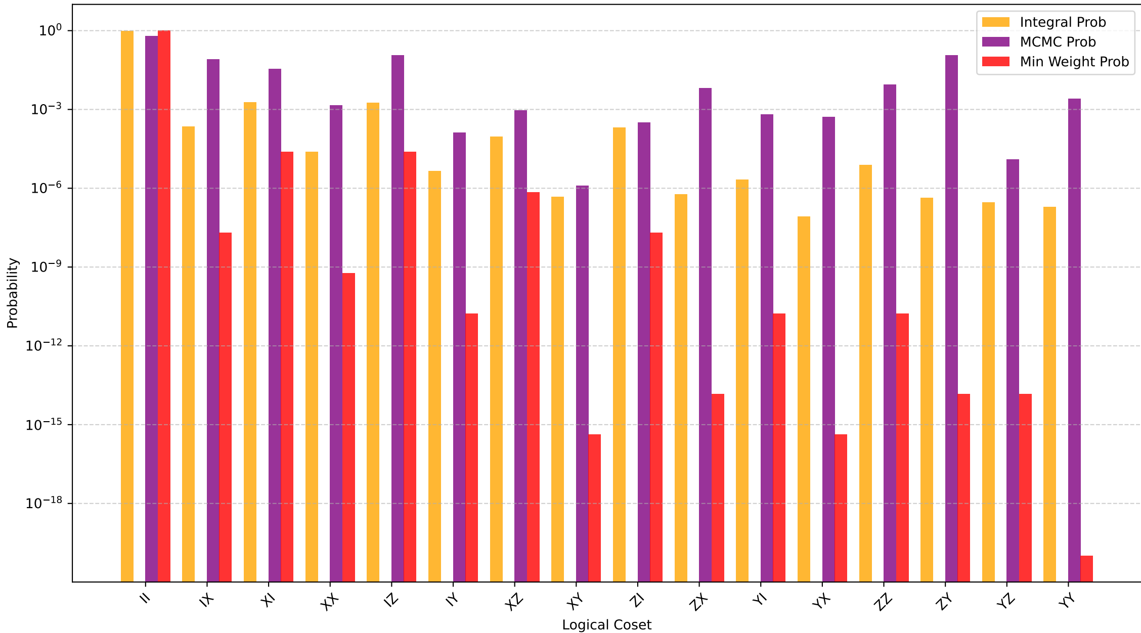
Coset Probabilities Proxies Comparison (L=5, p=0.08)
