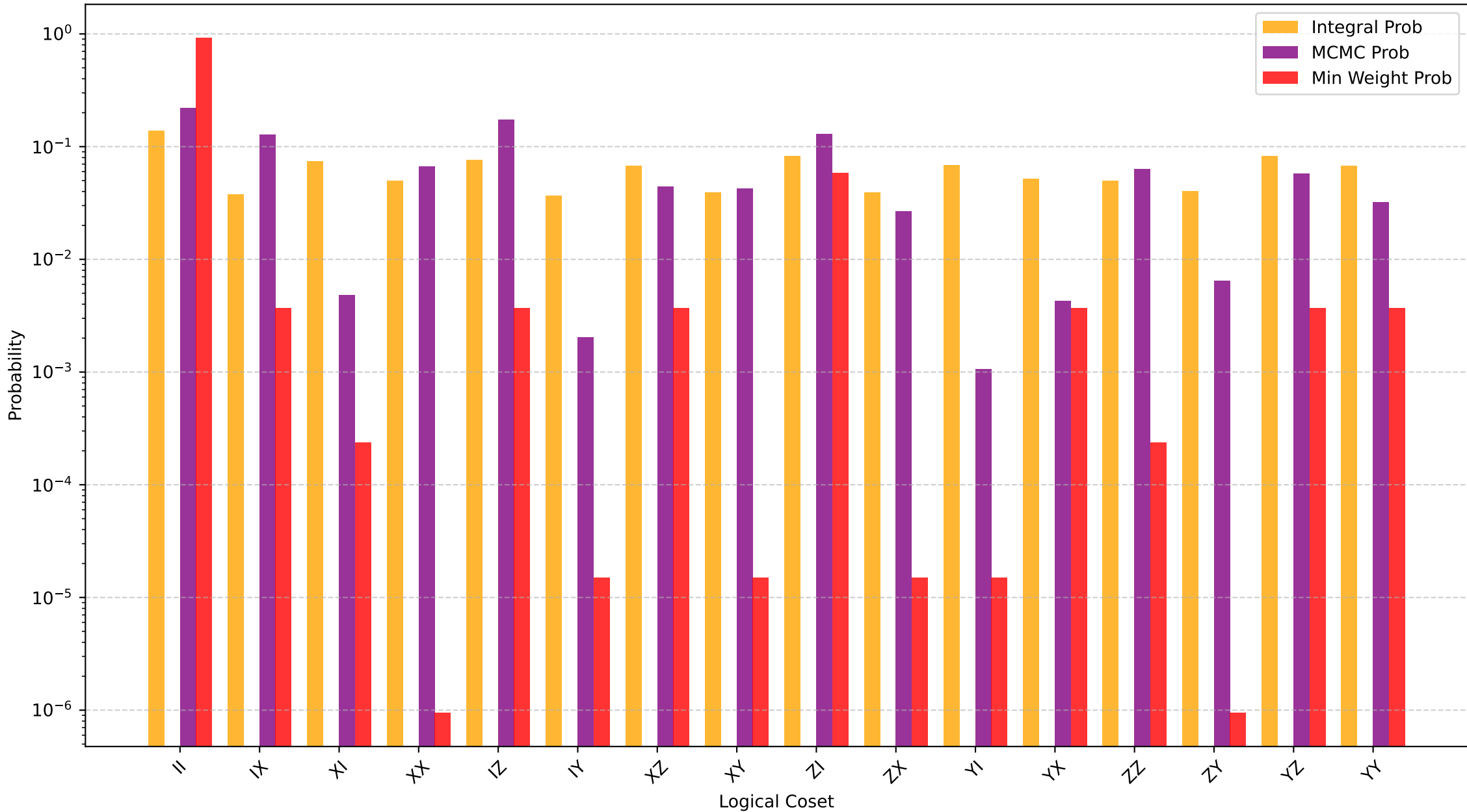
Coset Probabilities Proxies Comparison (L=5, p=0.16)
