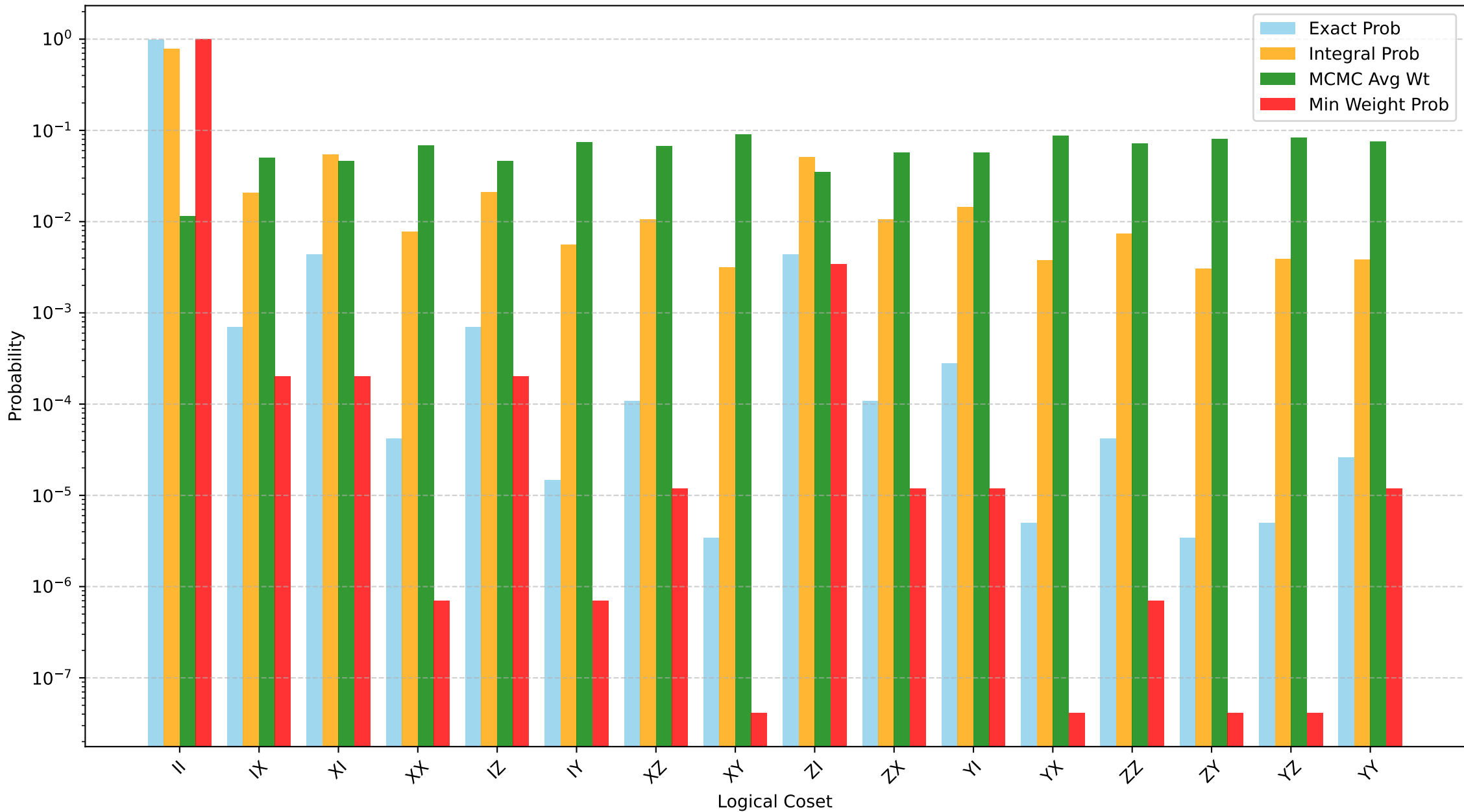
Coset Probabilities Proxies Comparison (L=3, p=0.15)
