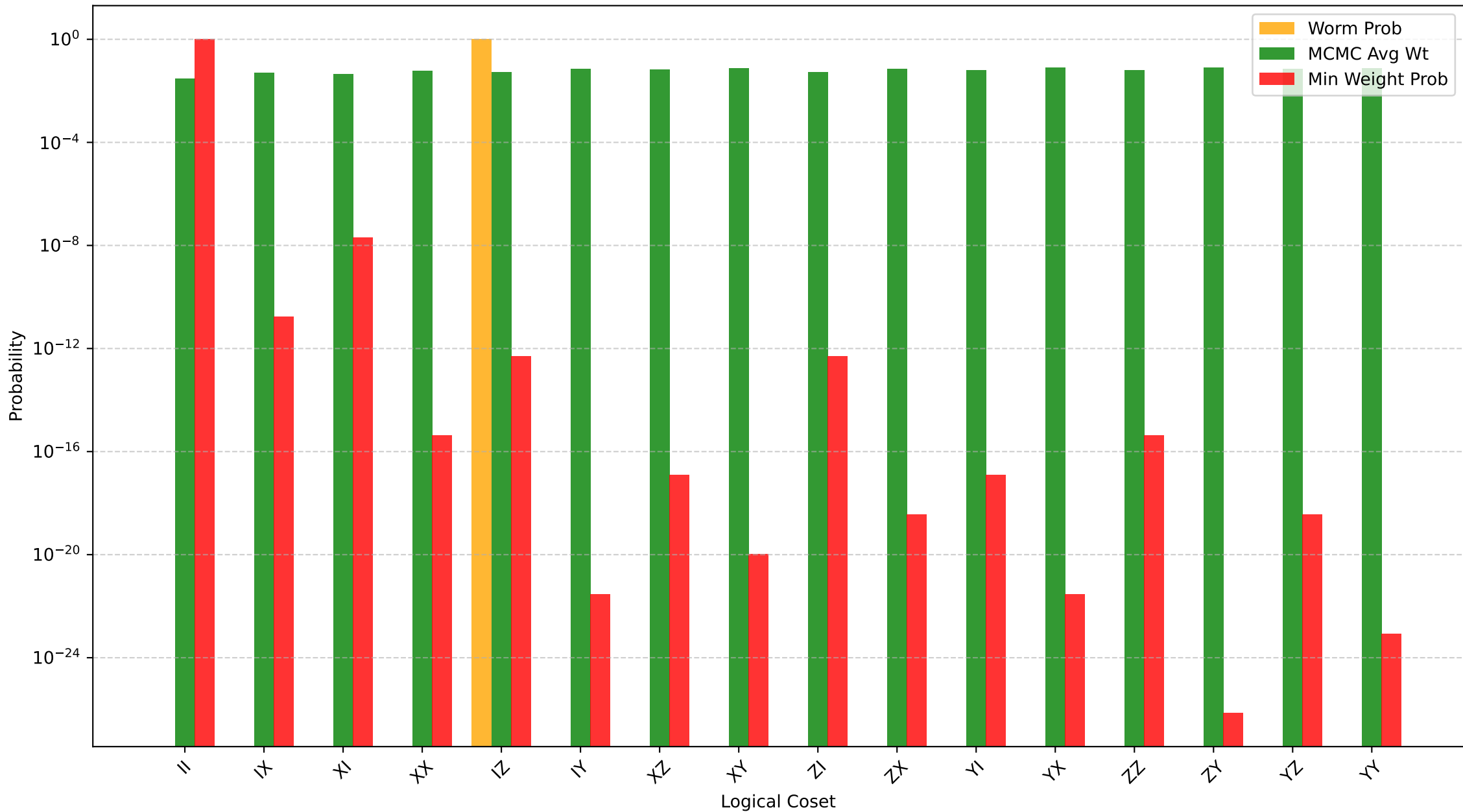
Coset Probabilities Proxies Comparison (L=8, p=0.08)
