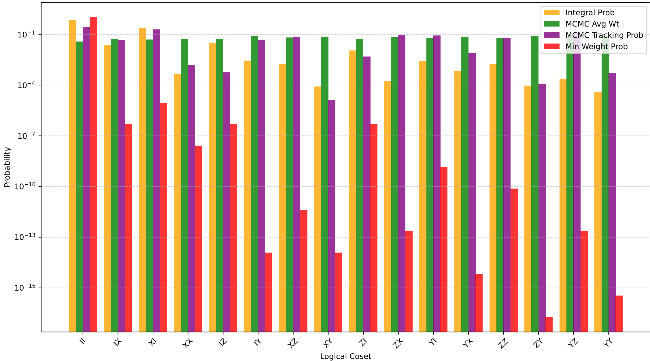
Coset Probabilities Proxies Comparison (L=8, p=0.14)
