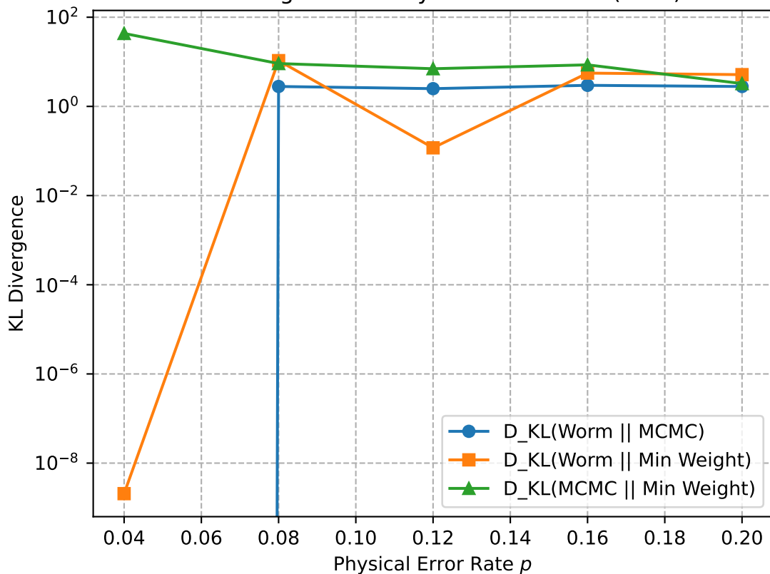
KL Divergence vs Physical Error Rate (Toric)
