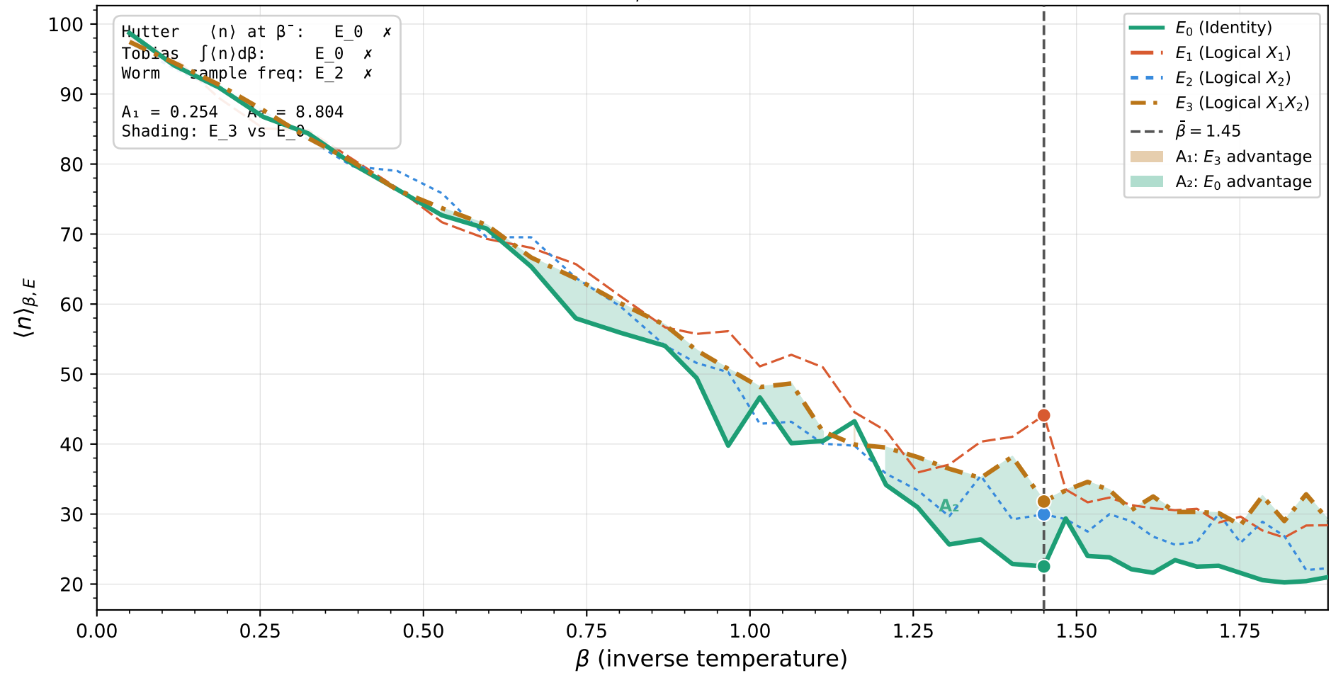
Toric code — \langle n \rangle_{\beta, E} curves ( L = 10 , p = 0.19 )
