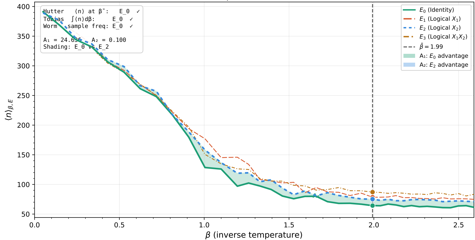
Toric code — \langle n \rangle_{\beta, E} curves ( L = 20 , p = 0.12 )
