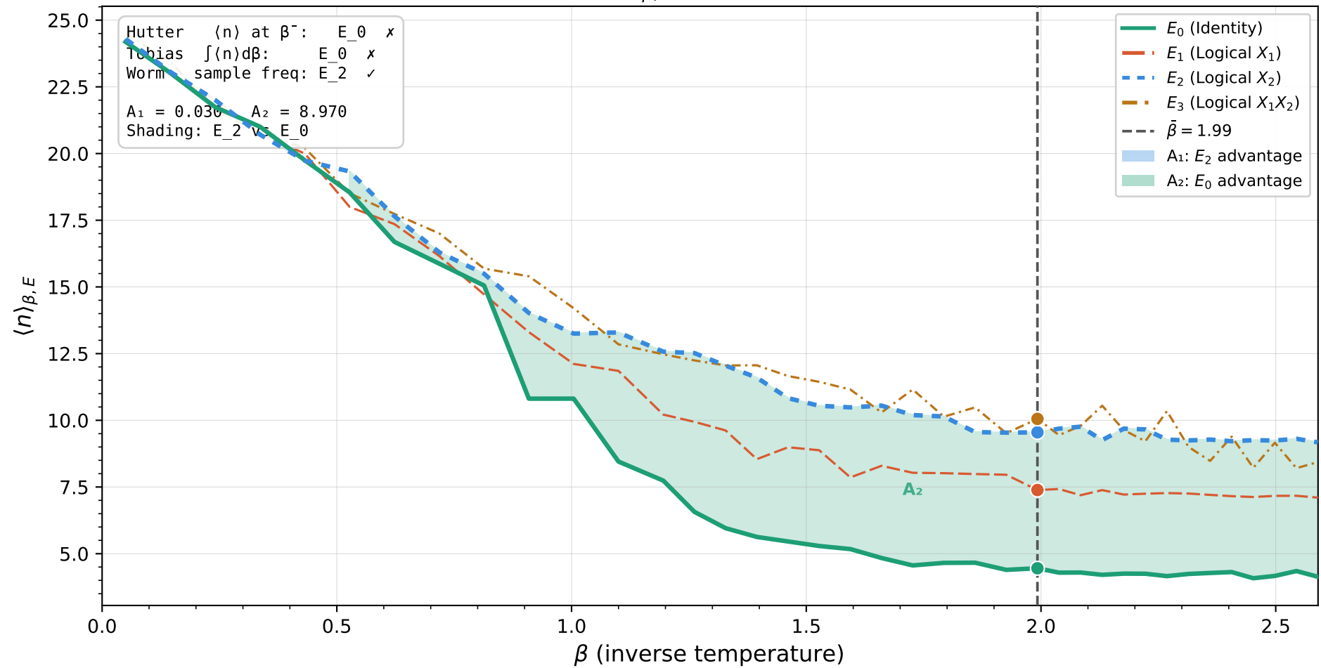
Toric code — \langle n \rangle_{\beta, E} curves ( L = 5 , p = 0.12 )
