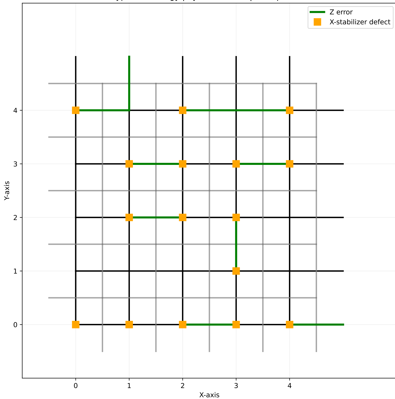
TypeG Pathology | hybrid: 0.2081 | L=5, p=0.15
