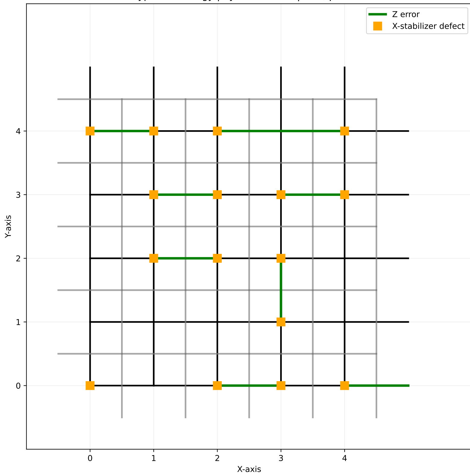
TypeG Pathology | hybrid: 0.9252 | L=5, p=0.15
