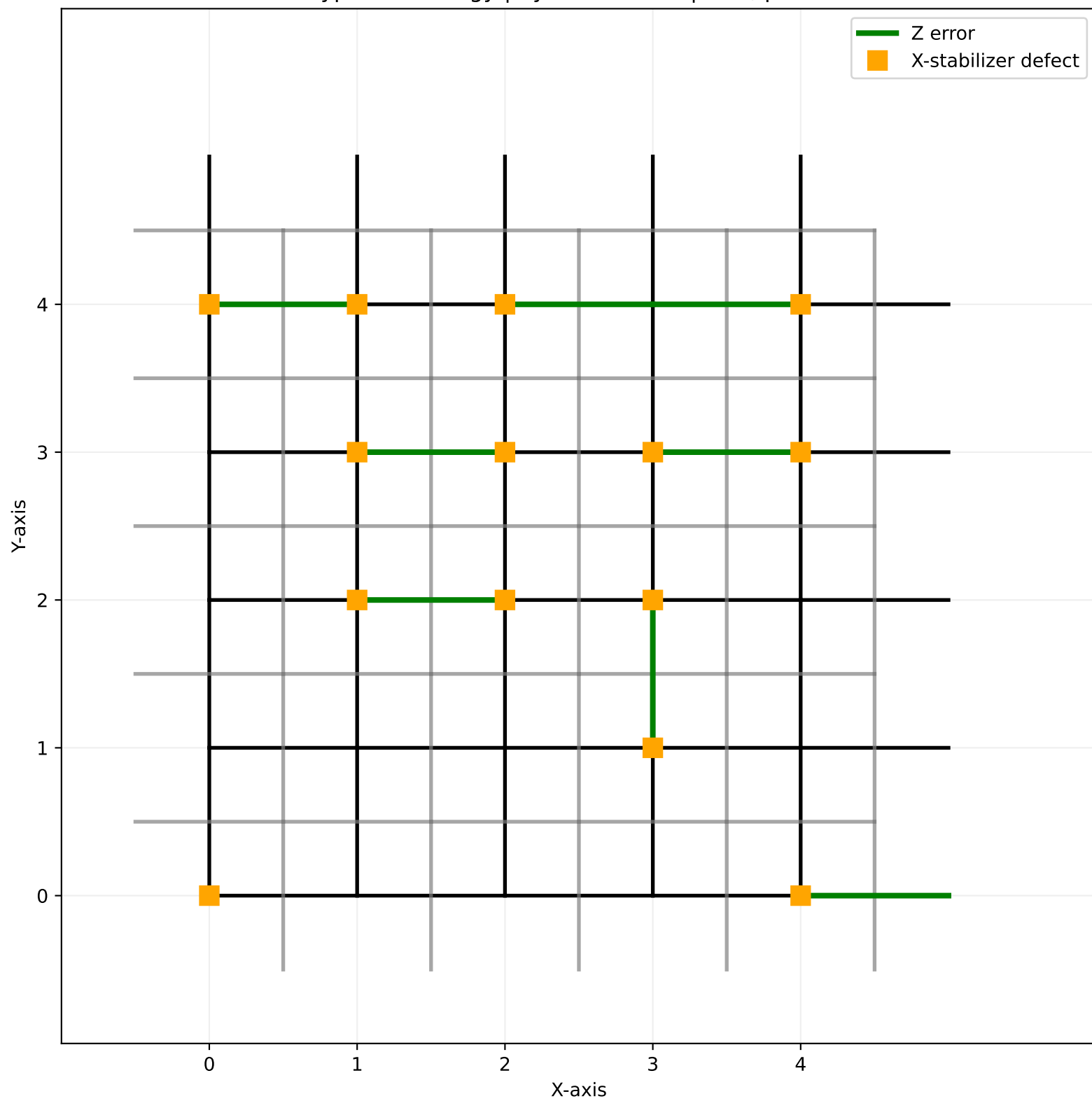
TypeG Pathology | hybrid: 0.8773 | L=5, p=0.15
