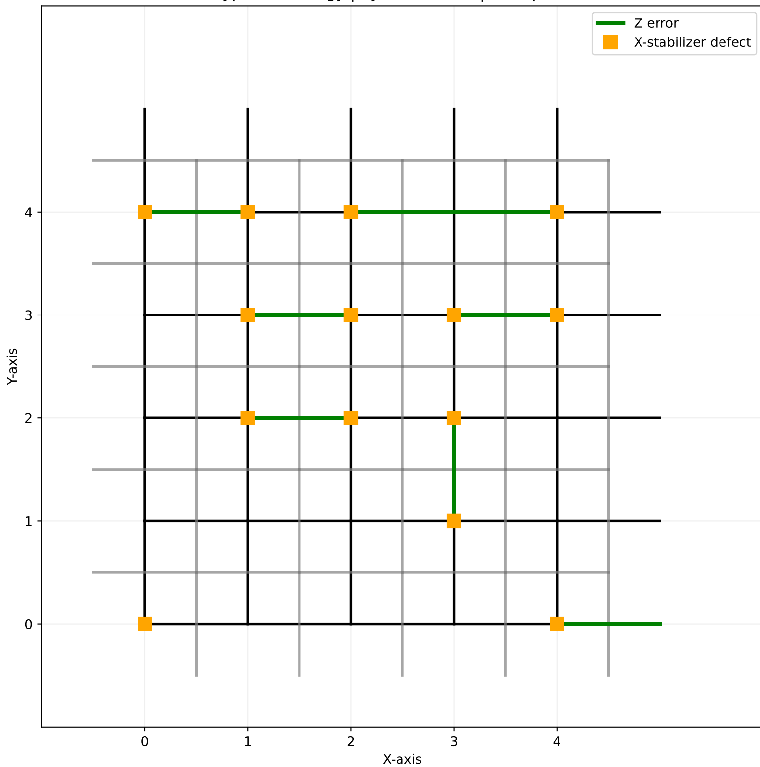
TypeG Pathology | hybrid: 0.3588 | L=5, p=0.15
