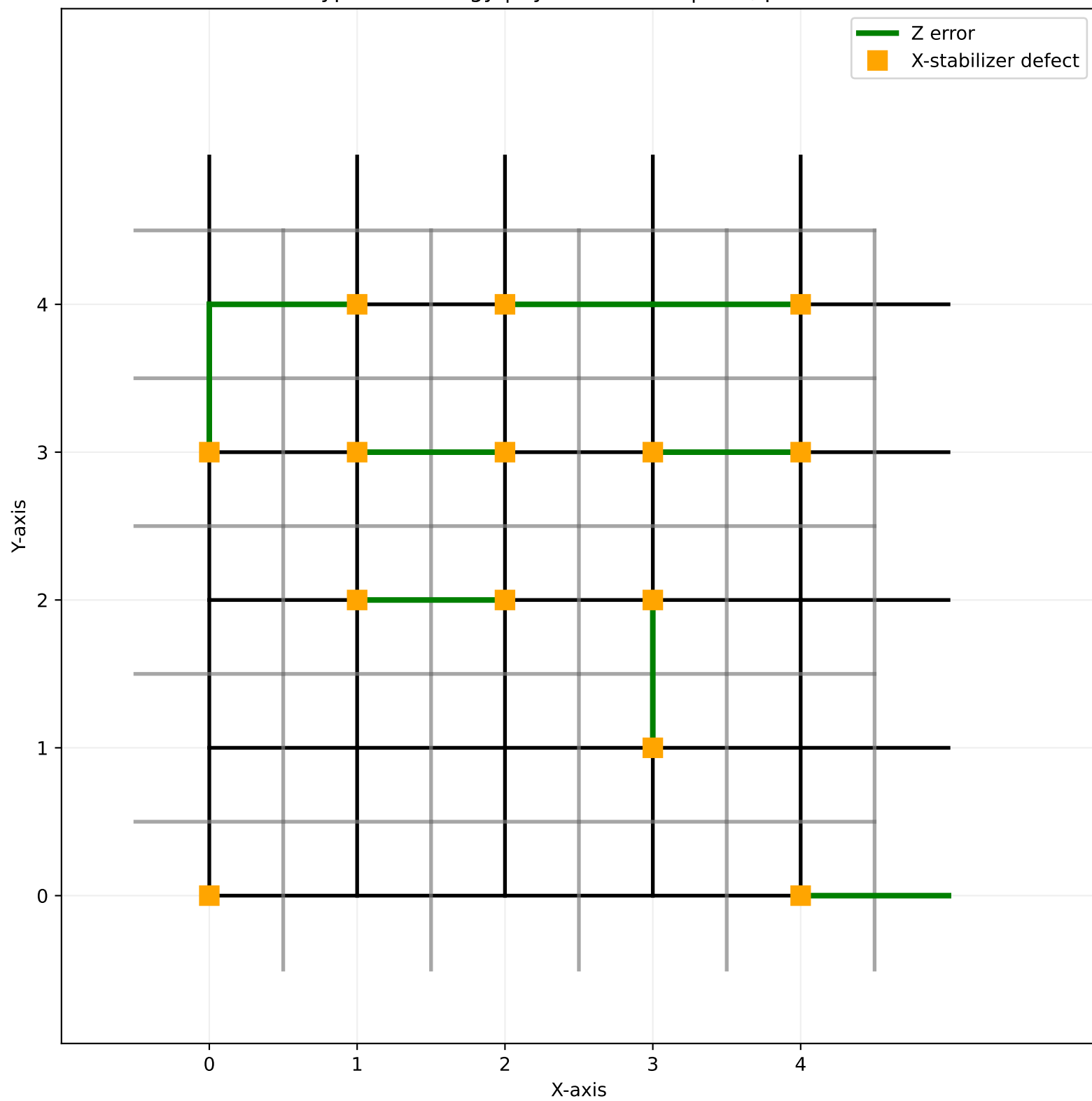
TypeG Pathology | hybrid: 2.0449 | L=5, p=0.15
