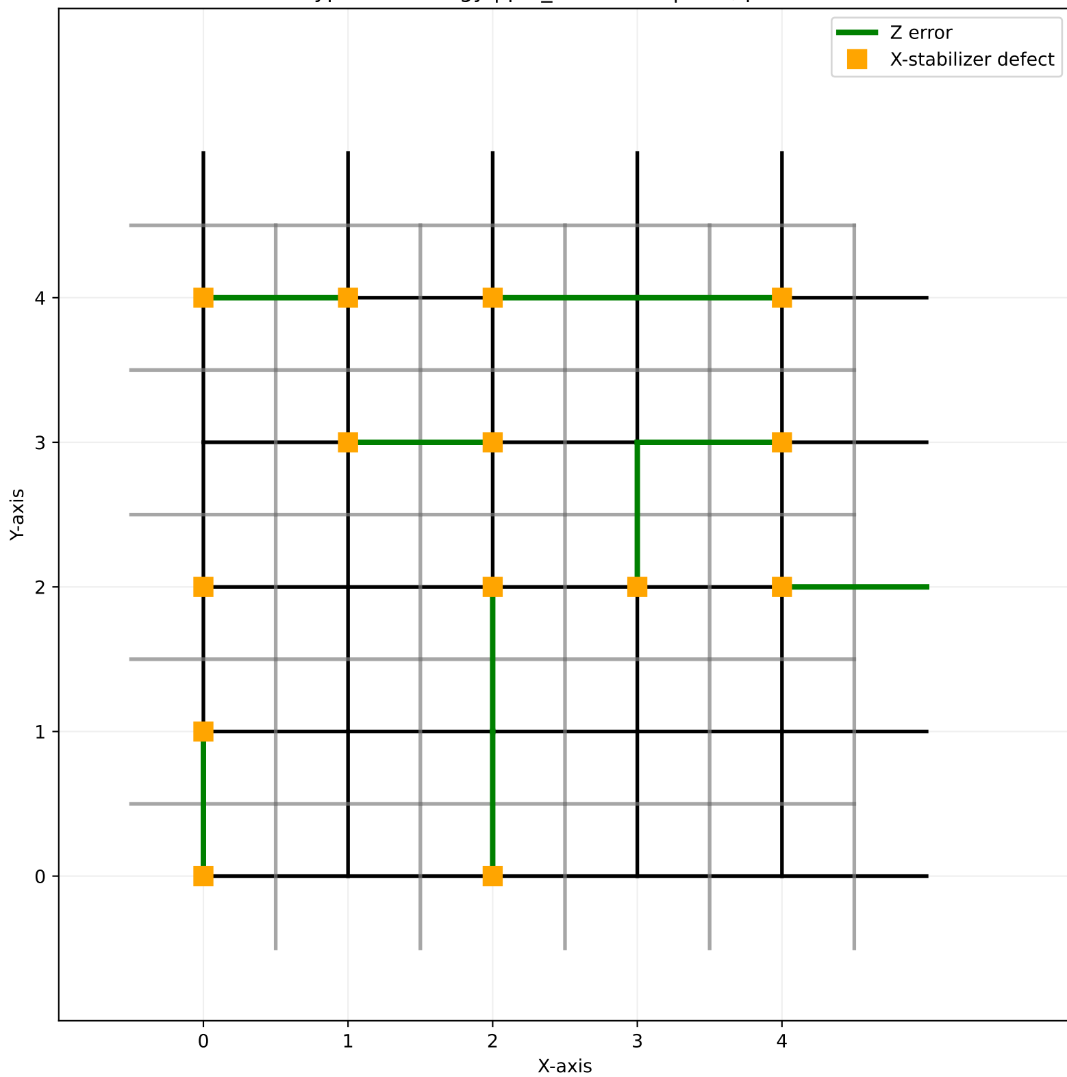
TypeG Pathology | \phi_1 : -3.0000 | L=5 , p=0.15
