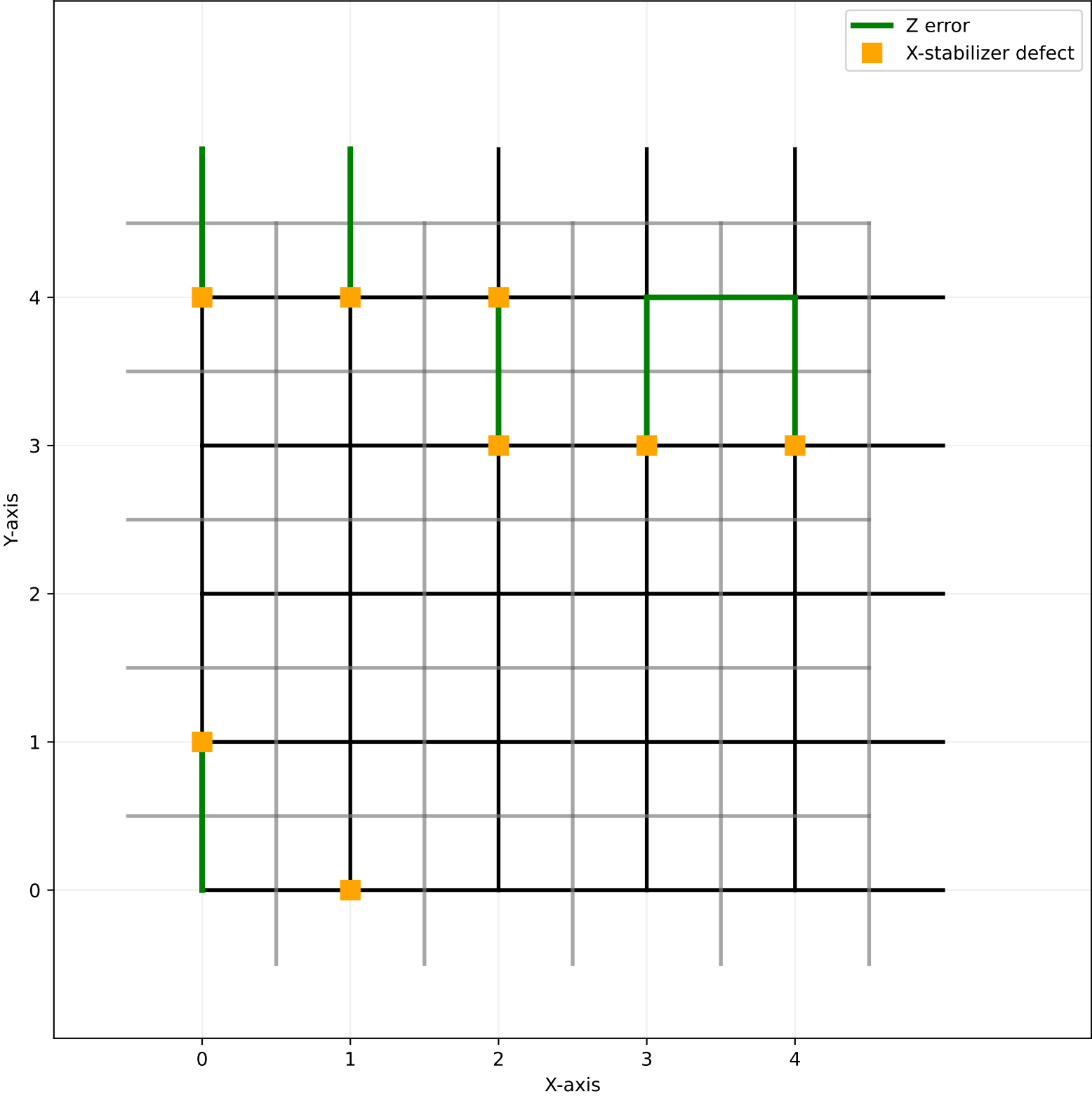
Type2 Pathology | \phi_2 : -1.2987 | L=5, p=0.15
