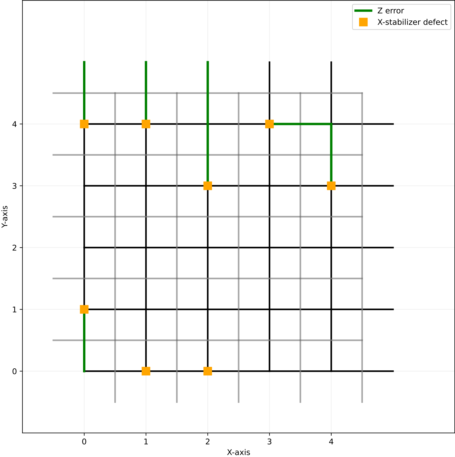
Type2 Pathology | \phi_2 : -0.5898 | L=5, p=0.15
