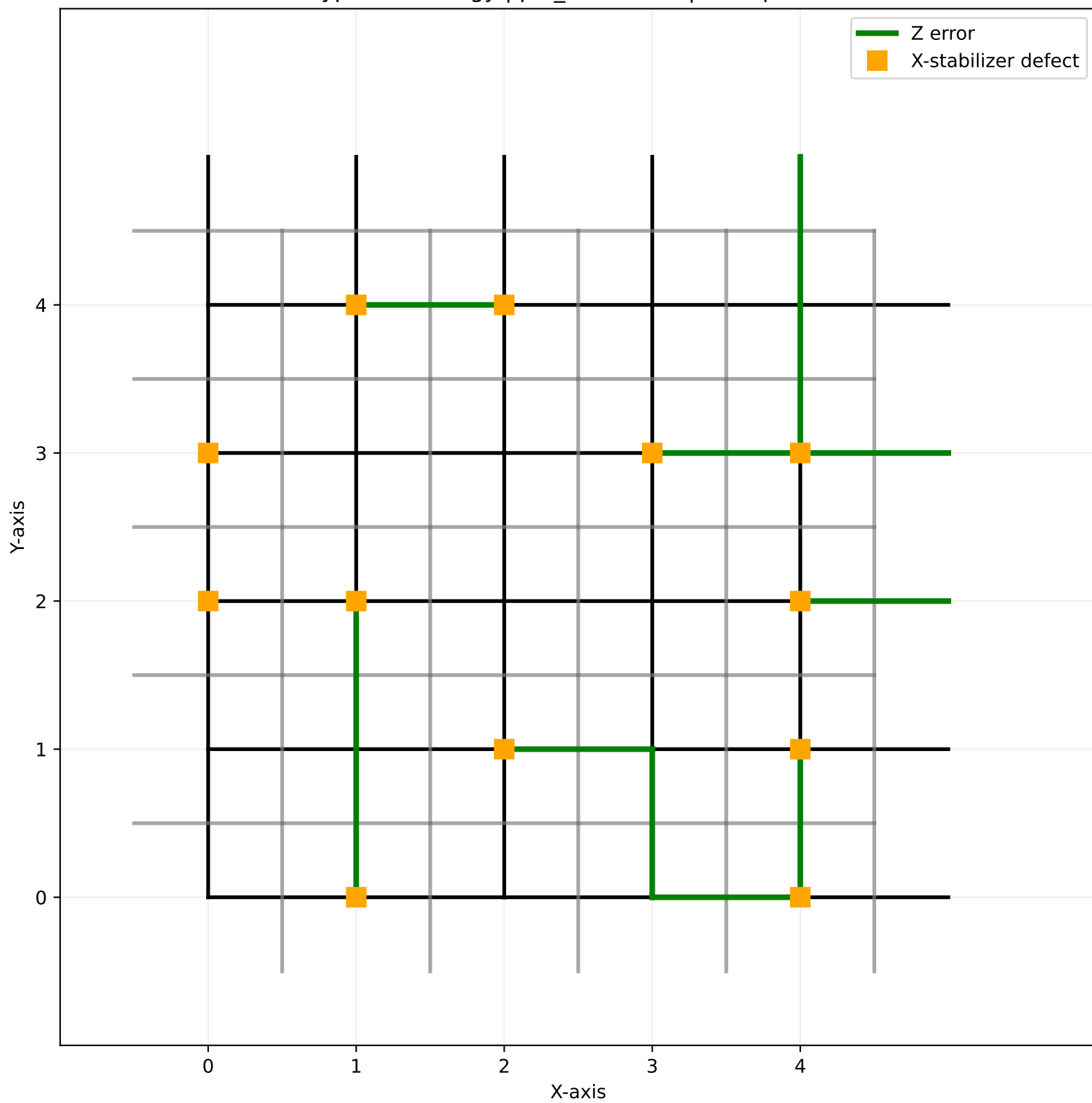
TypeG Pathology | \phi_3 : -0.6920 | L=5 , p=0.15
