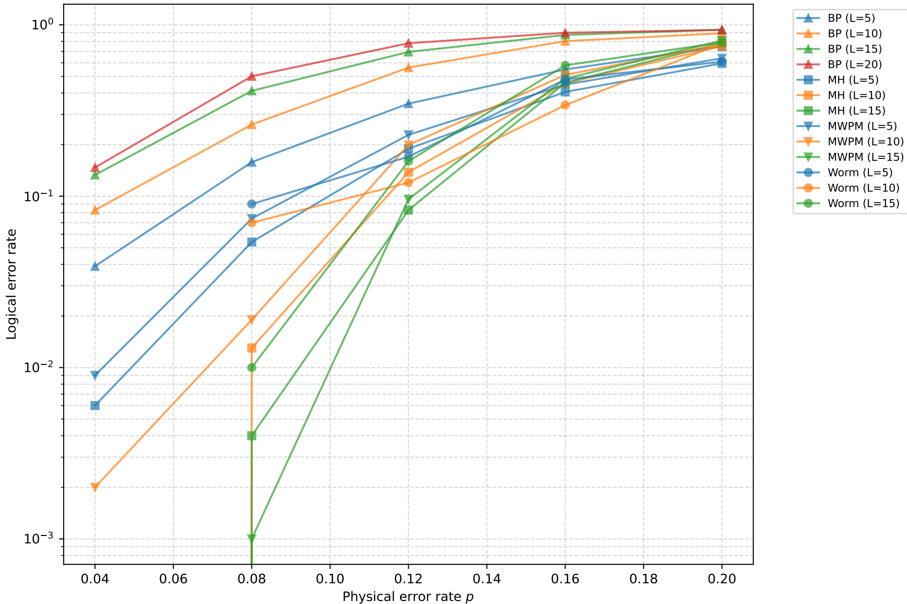
Threshold Comparison: BP vs MH vs MWPM vs Worm
