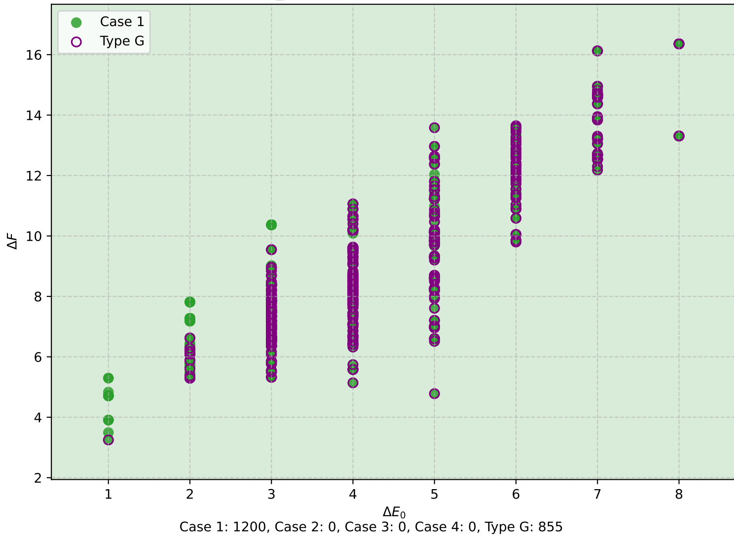
\Delta F vs \Delta E_0 for pathology candidate syndromes
