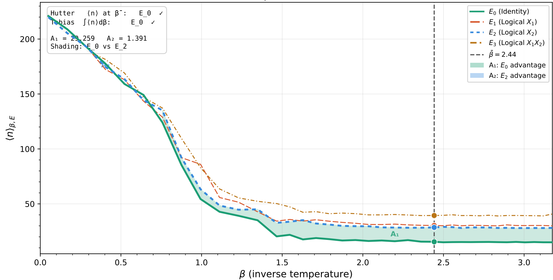
Toric code — \langle n \rangle_{\beta, E} curves ( L = 15 , p = 0.08 )
