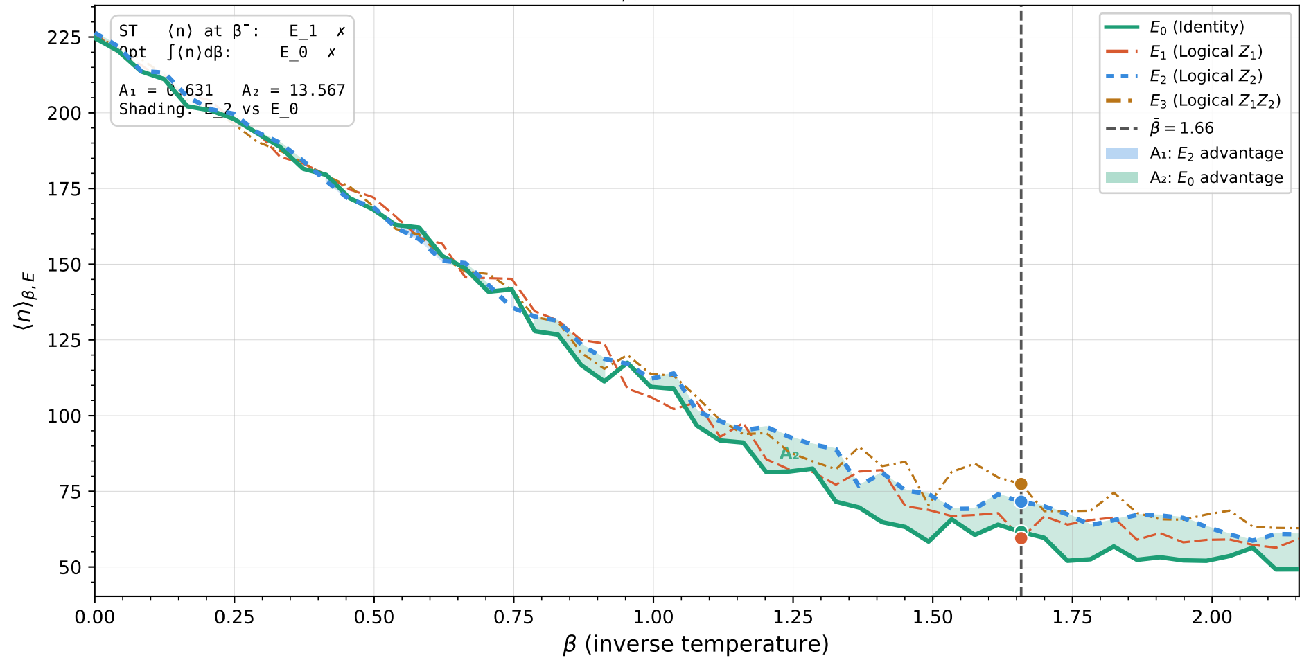
Toric code — \langle n \rangle_{\beta, E} curves ( L = 15 , p = 0.16 )
