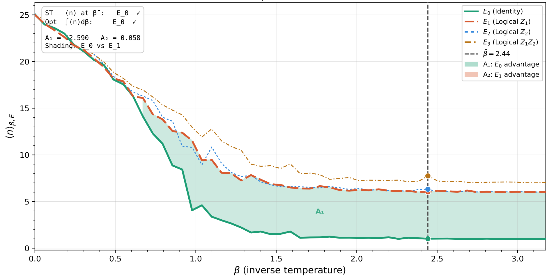
Toric code — \langle n \rangle_{\beta, E} curves ( L = 5 , p = 0.08 )
