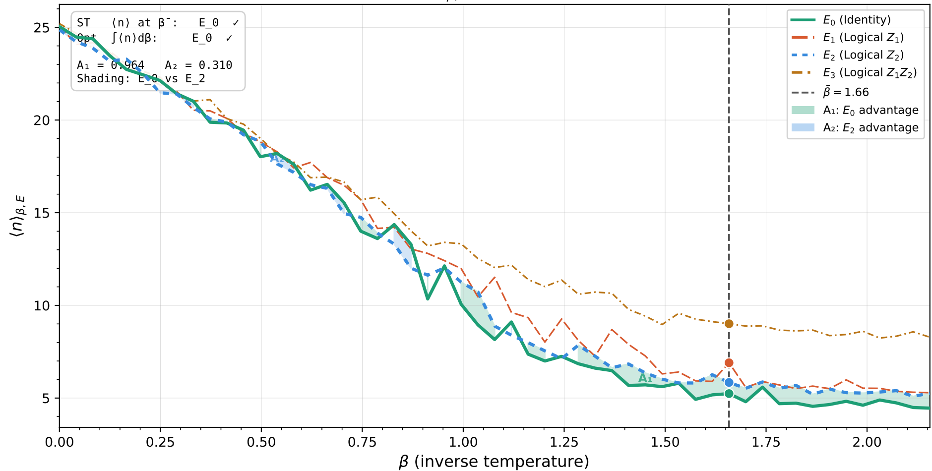
Toric code — \langle n \rangle_{\beta, E} curves ( L = 5 , p = 0.16 )
