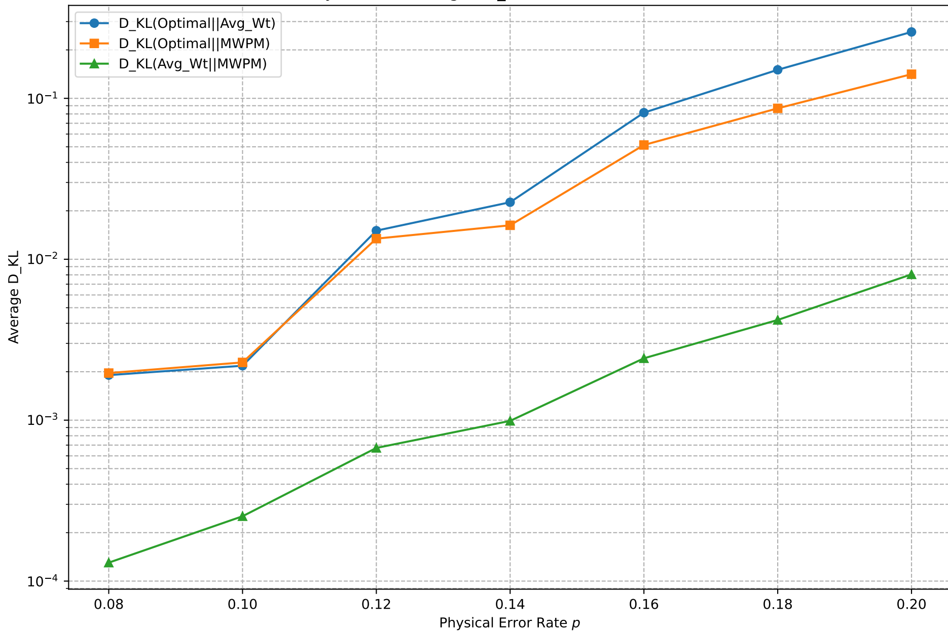
Syndrome-Averaged D_KL via MBAR (Toric, L=5)
