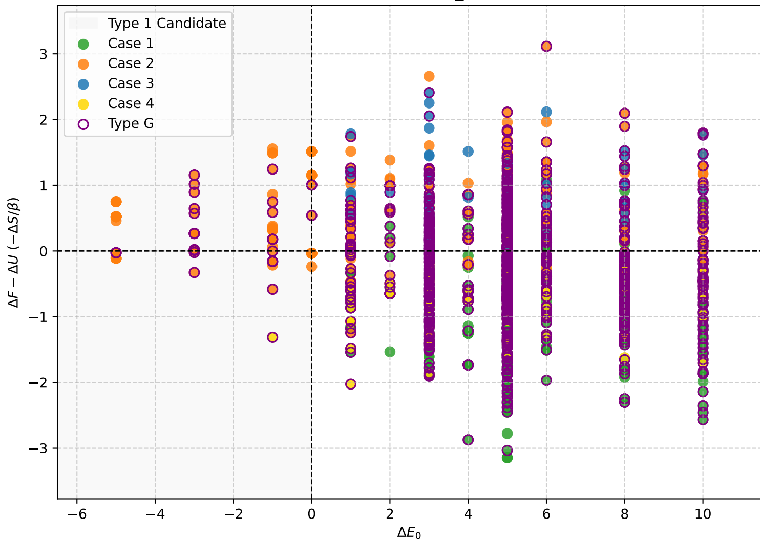
\Delta F - \Delta U vs \Delta E_0
