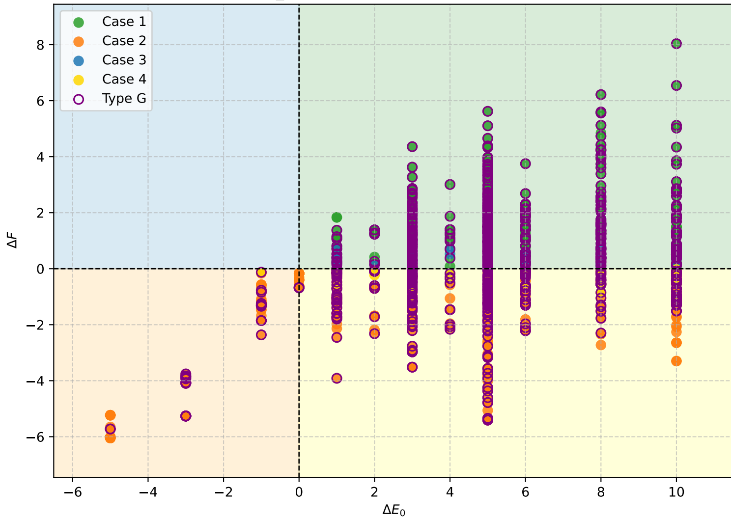
\Delta F vs \Delta E_0 for pathology candidate syndromes
