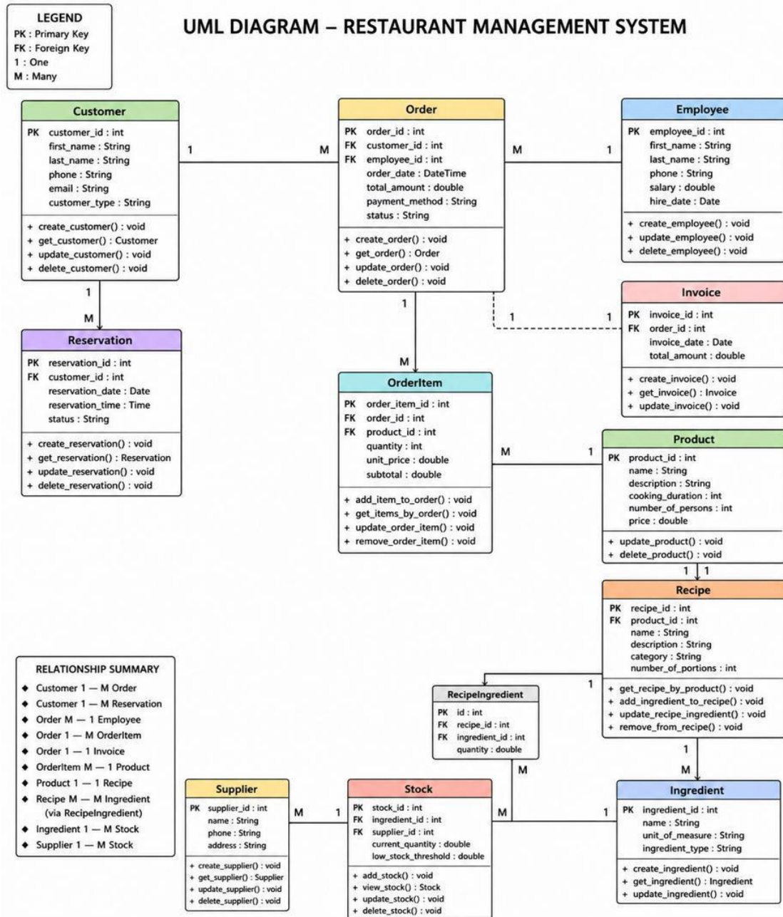
Figure 3: Class model
