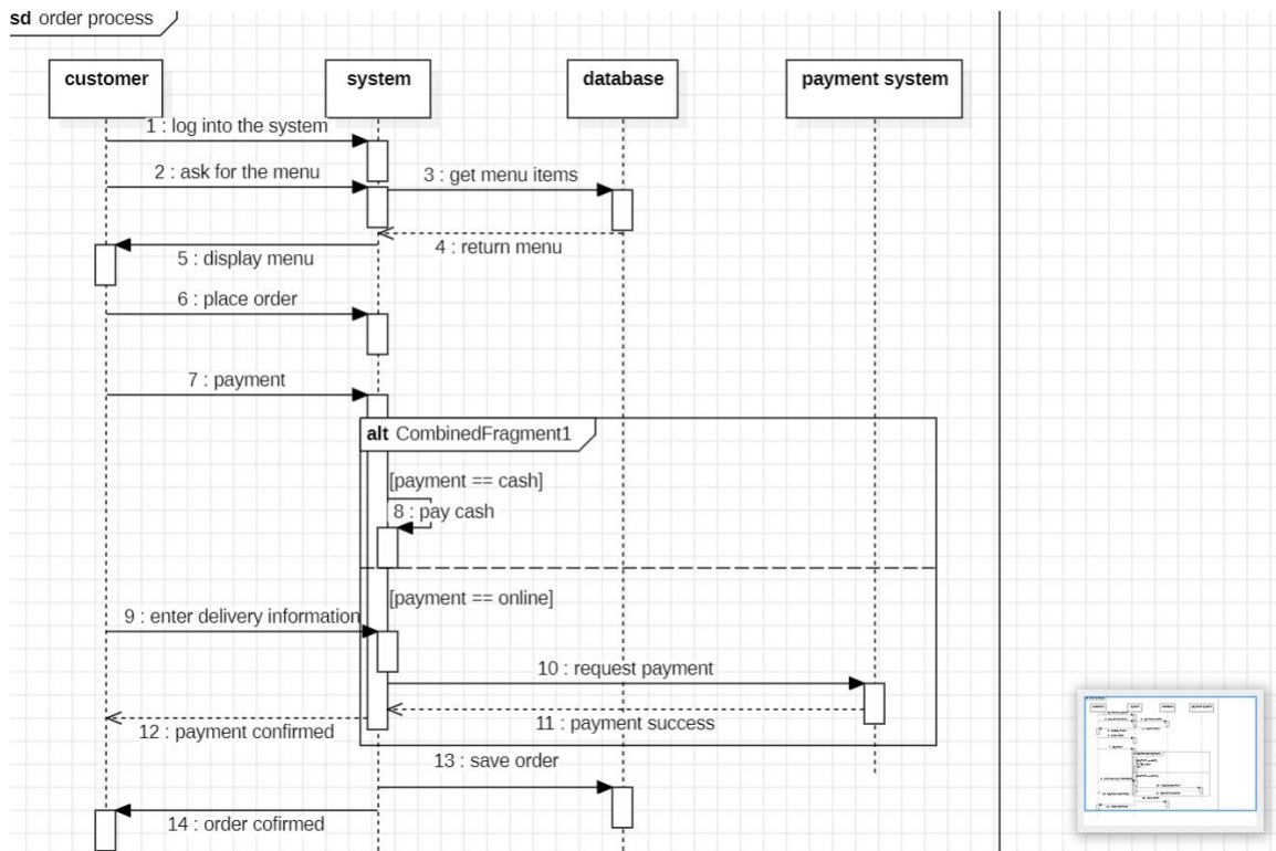
Figure 5: Sequence Diagram
