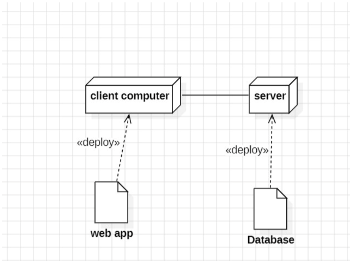
Figure 4: Deployment Diagram
