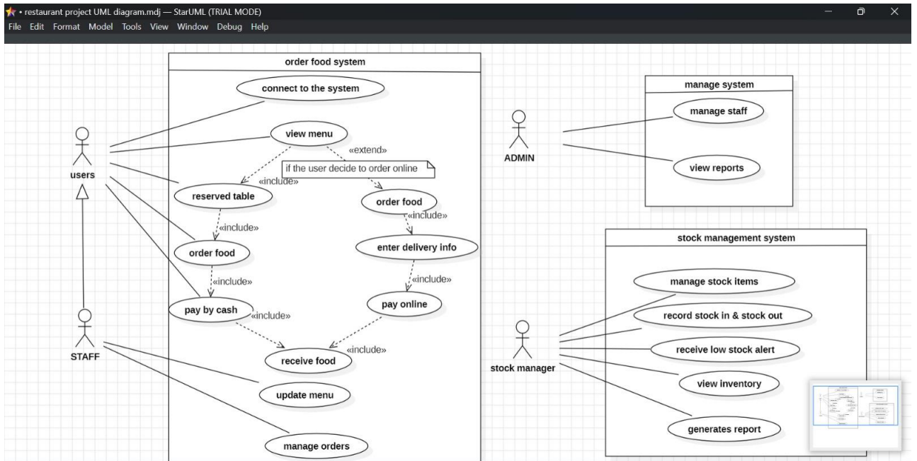
Figure h: User case diagram
