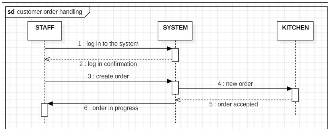
Figure j.: Sequence diagram continuity
