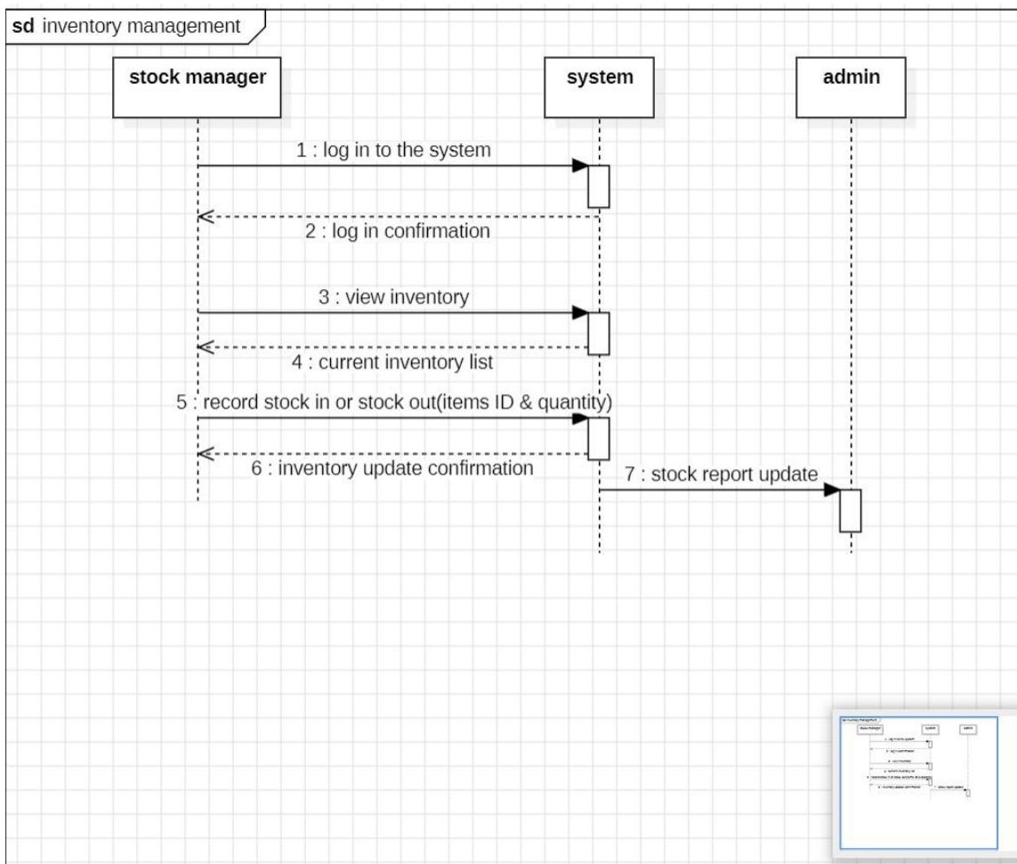
Figure k: Sequence diagram end
