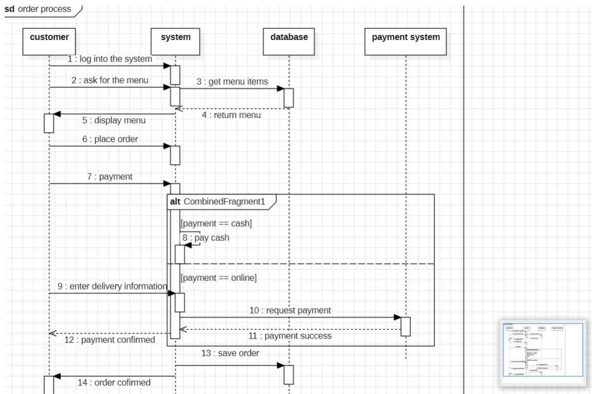
Figure i.1: Sequence Diagram
