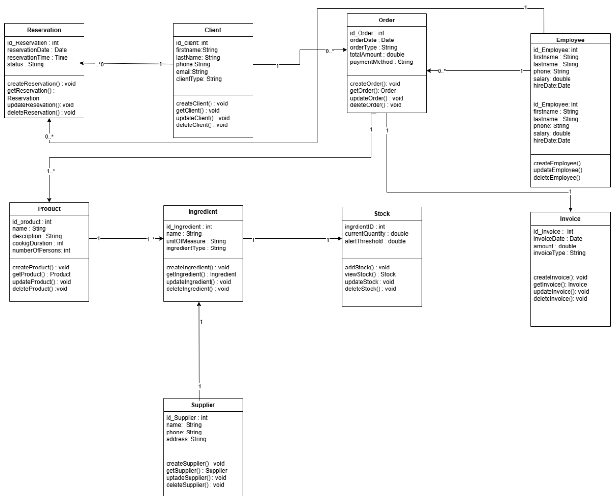
Figure g: Class model
