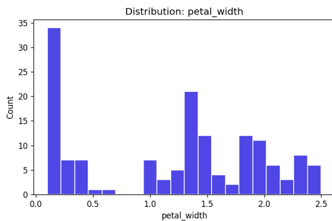
Figure 2: Histogram of petal_width
