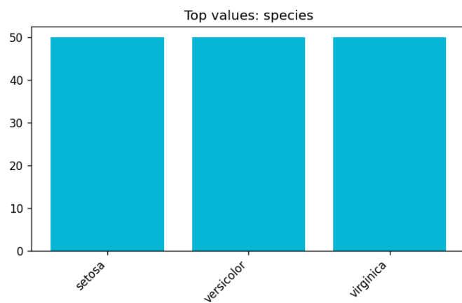
Figure 3: Top categories in species
