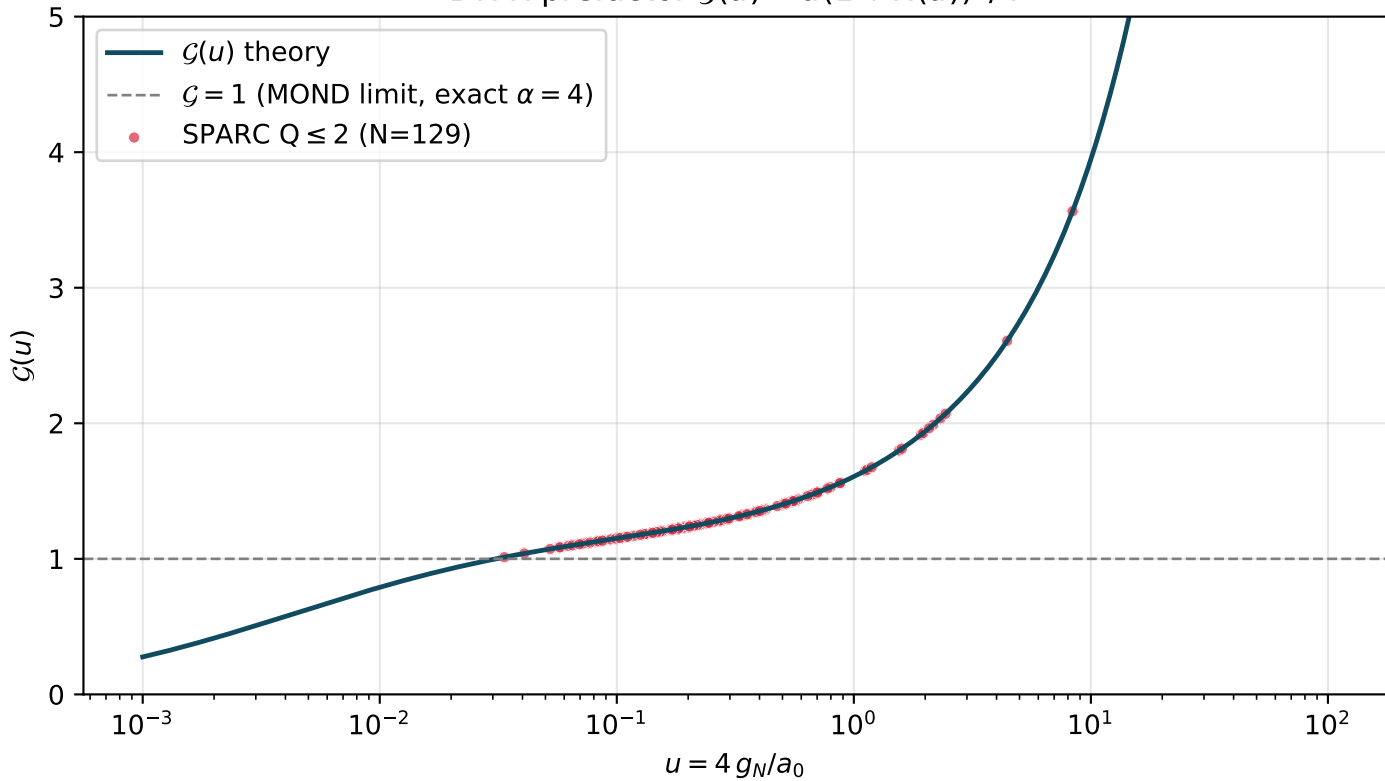
BTFR prefactor \mathcal{G}(u) = u(1 + R(u))^2/4
