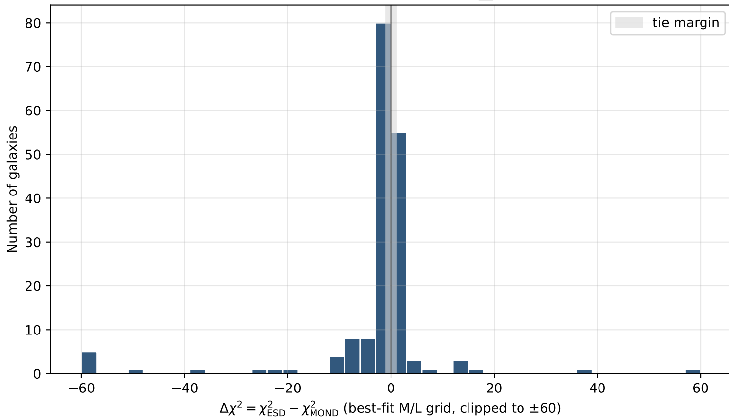
Per-galaxy \Delta\chi^2 distribution (N=175, \sum\Delta\chi^2 = -843 )
