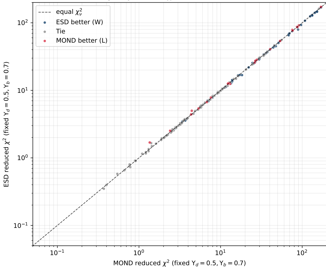
Per-galaxy reduced \chi^2 : ESD vs MOND (N=175)
