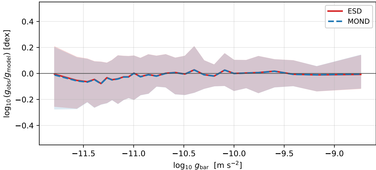
Study 05: RAR log-residuals (median + 16/84 percentile band)
