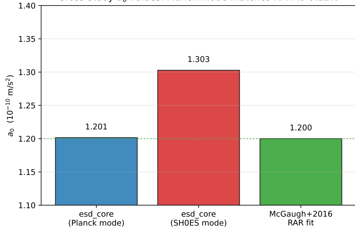
Cross-study a_0 values: Planck mode matches RAR to 0.12%
