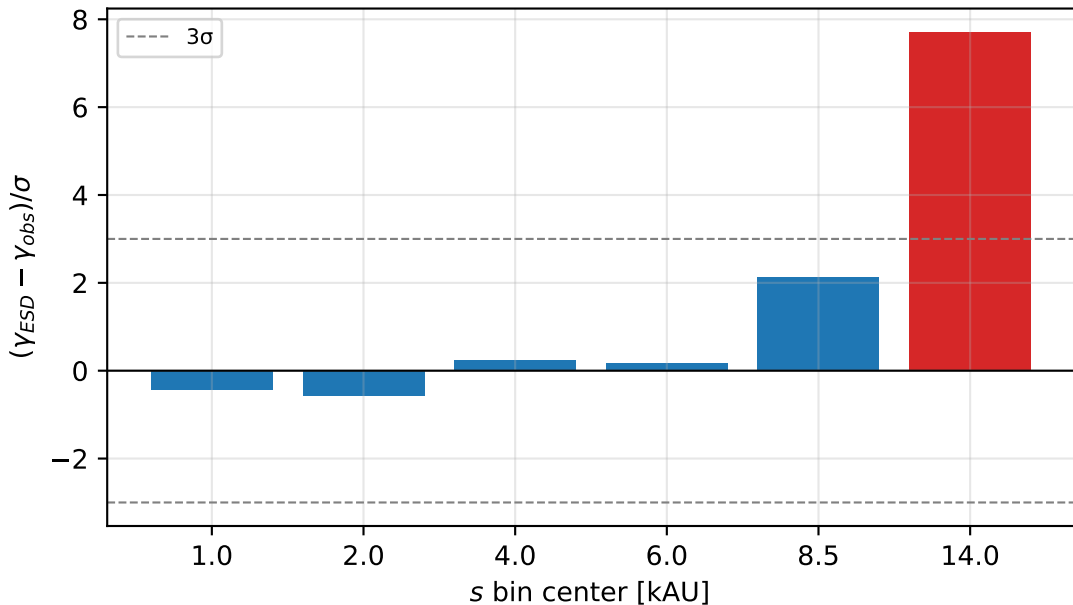
ESD residuals vs Chae 2023 (blue: intermediate, red: deep)
