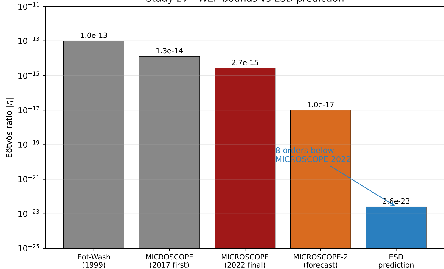
Study 27 - WEP bounds vs ESD prediction
