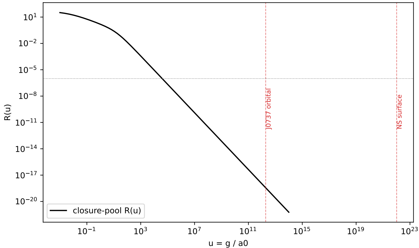
B03: closure-pool kernel suppression at pulsar scales
