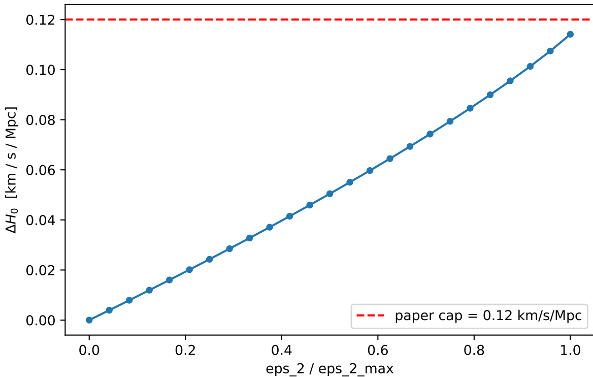
Disformal channel contribution to H_0 shift
