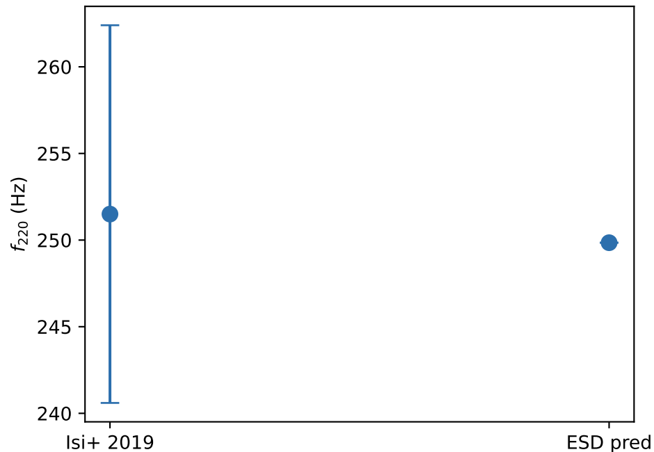
GW150914 220-mode frequency
