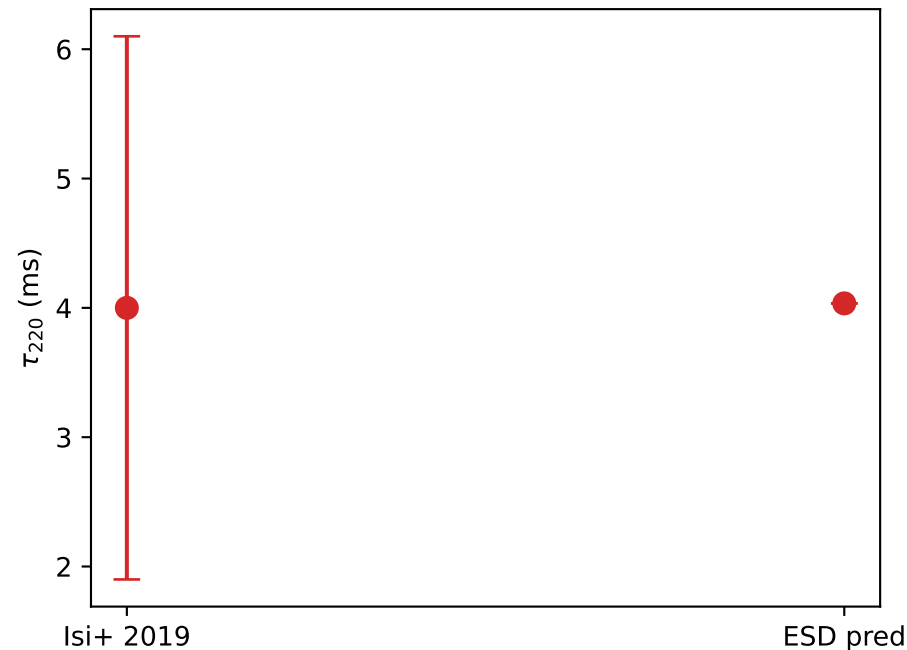
GW150914 220-mode damping time
