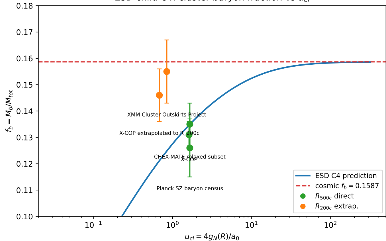
ESD child C4: cluster baryon fraction vs u_{cl}
