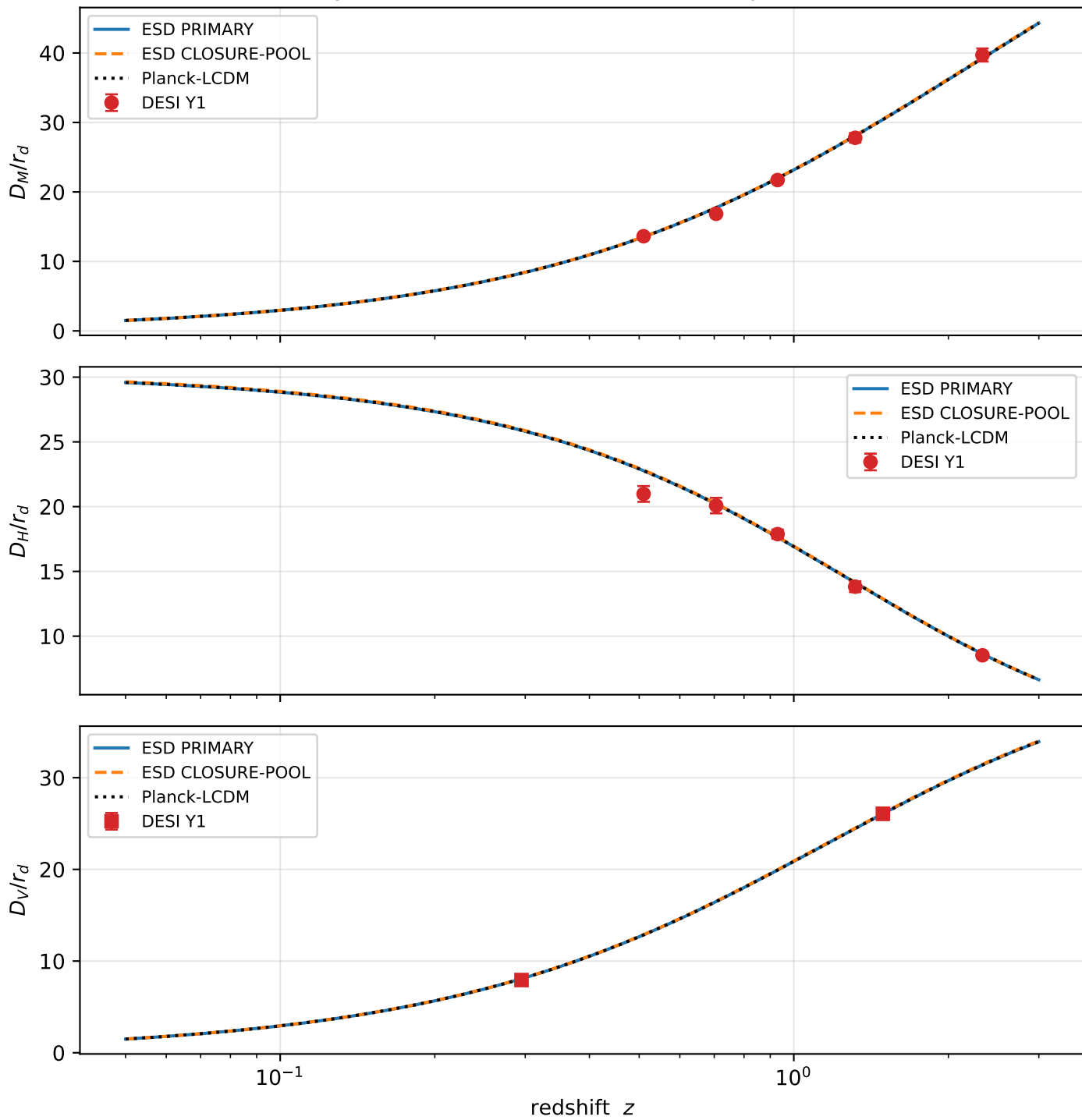
Study 07: DESI Y1 BAO vs framework predictions
