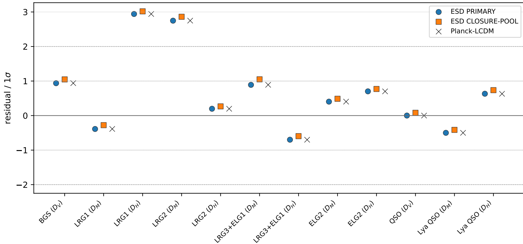
Study 07: per-tracer residuals across cosmologies ( H_0=67.36 )
