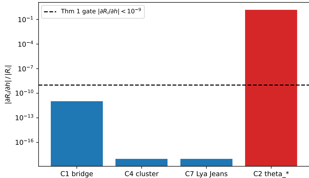
h-blindness theorem (ESD-distinctive children, blue)
