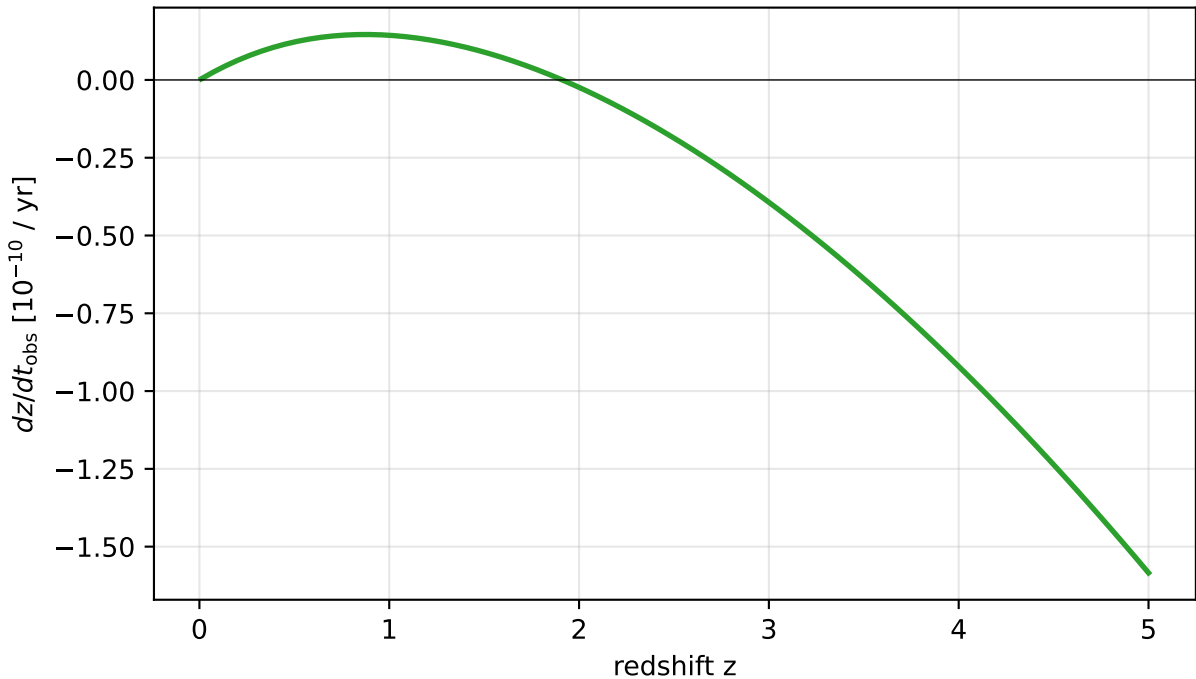
Sandage redshift drift — ESD predicts standard LambdaCDM curve
