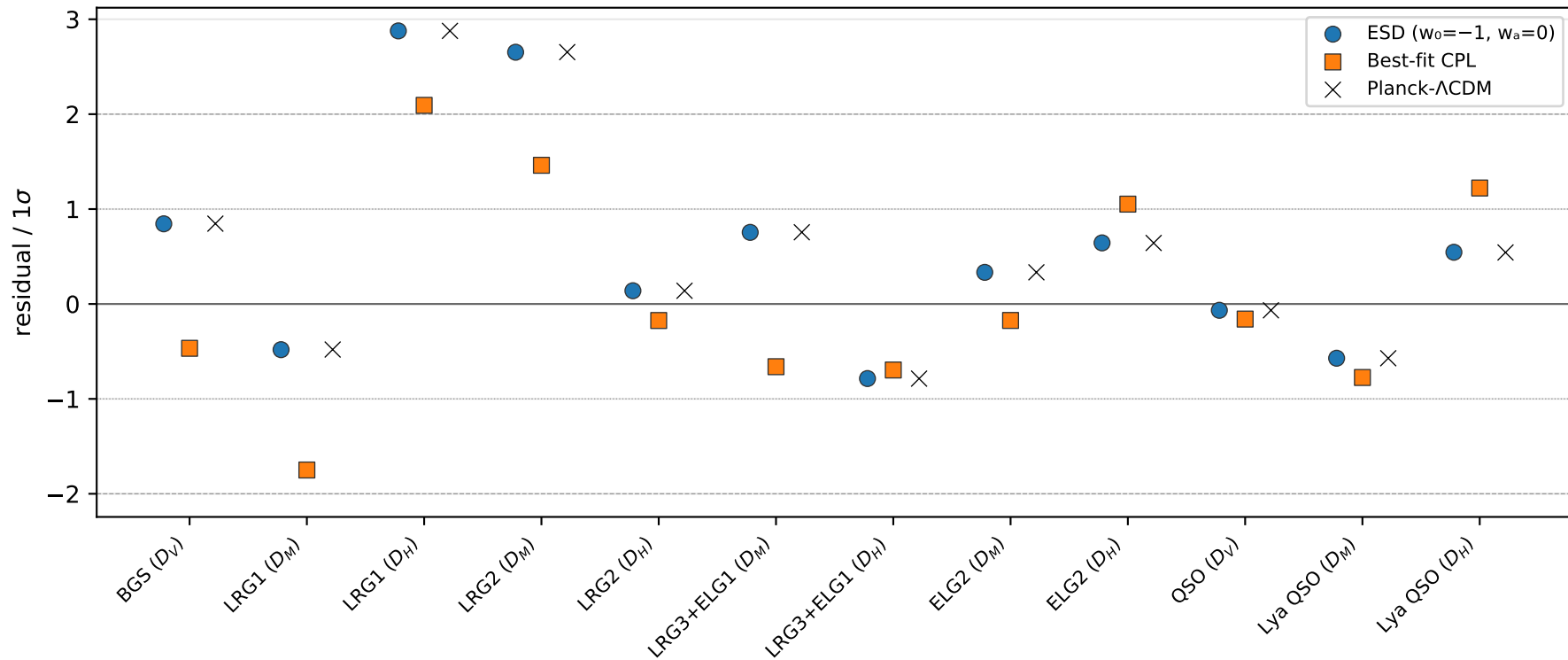
Study 22: DESI Y1 BAO per-tracer residuals ESD ( w_0=-1 , w_a=0 ) vs best-fit CPL vs Planck- \Lambda CDM
