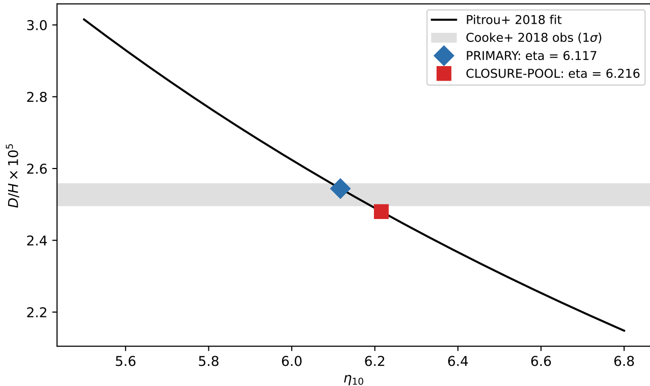
Study E09: BBN D/H under both Identity B readings
