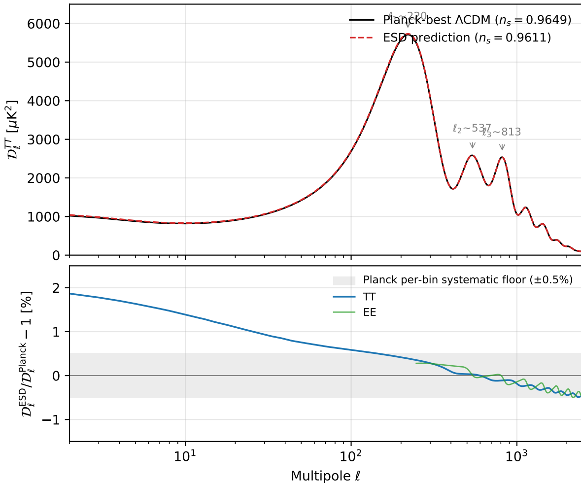
Framework vs Planck-best CMB anisotropy spectra
