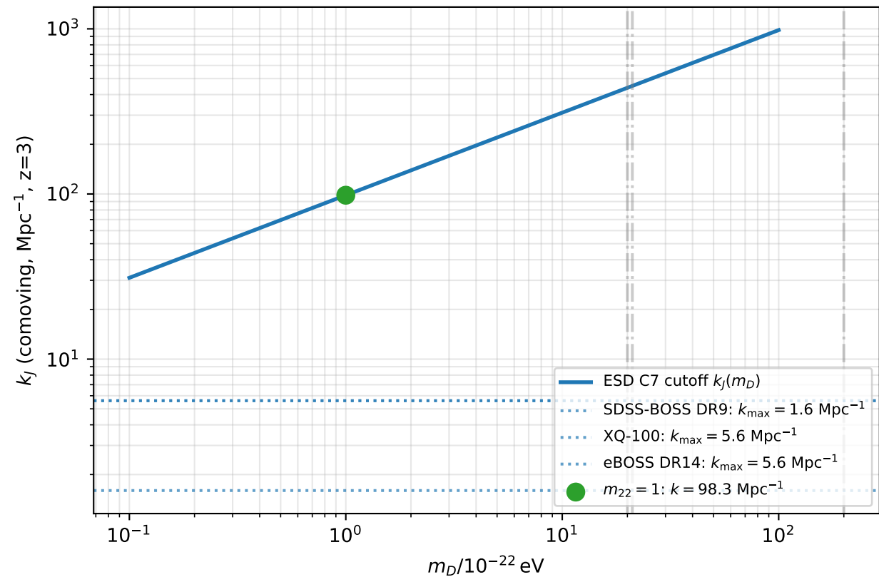
Lyman- \alpha probe range vs framework cutoff
