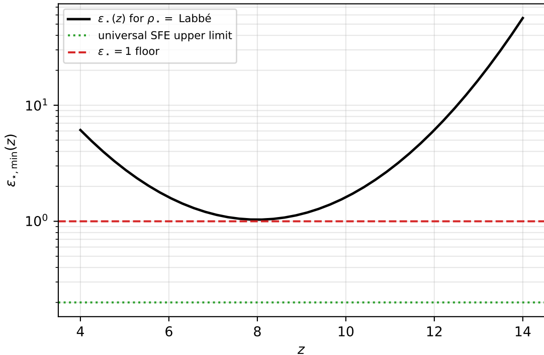
\varepsilon^*_{\text{min}} vs z with toy f_{\text{collapse}}(z) (BK23 normalization)
